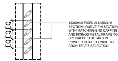
TYPICAL UNIT BALCONY LOUVRE SCREEN - DETAIL A
