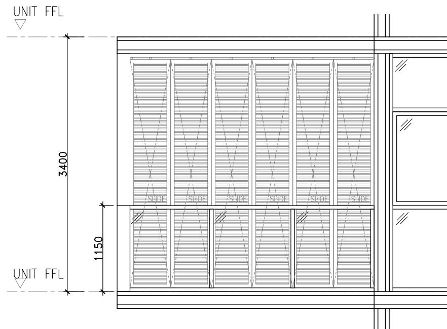
TYPICAL UNIT BALCONY LOUVRE SCREEN - ELEVATION
