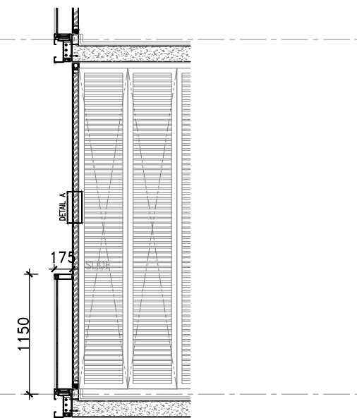
TYPICAL UNIT BALCONY LOUVRE SCREEN - SECTION
